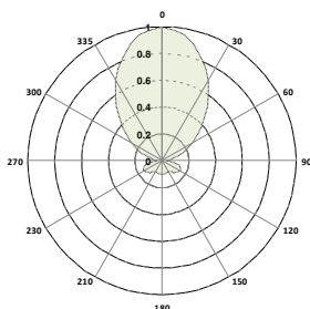
80 Mhz E plane
