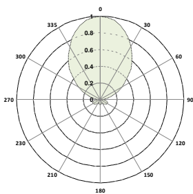
60 Mhz E plane
