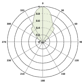
1000 Mhz E plane
