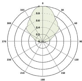
1000 Mhz H plane
