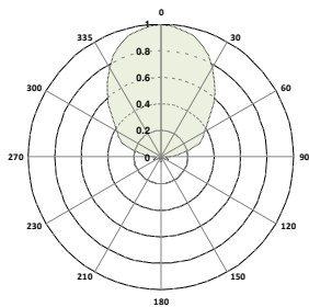
400 Mhz H plane
