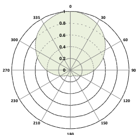
470 Mhz E plane
