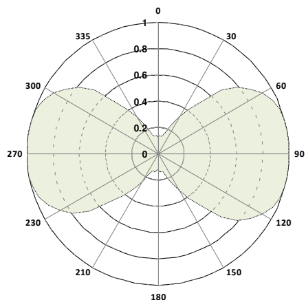
98 Mhz E plane
