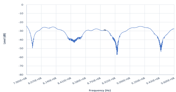
Return loss
